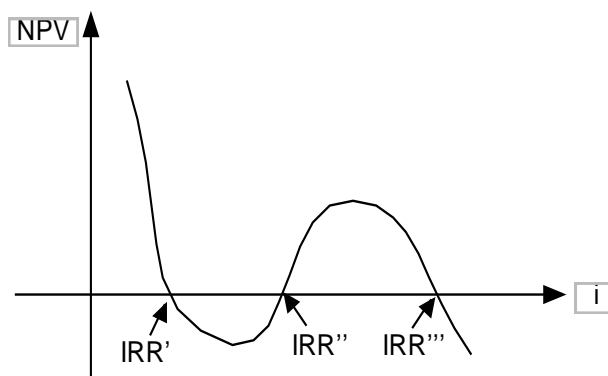
Figure VIII.4 Multiple IRRs
